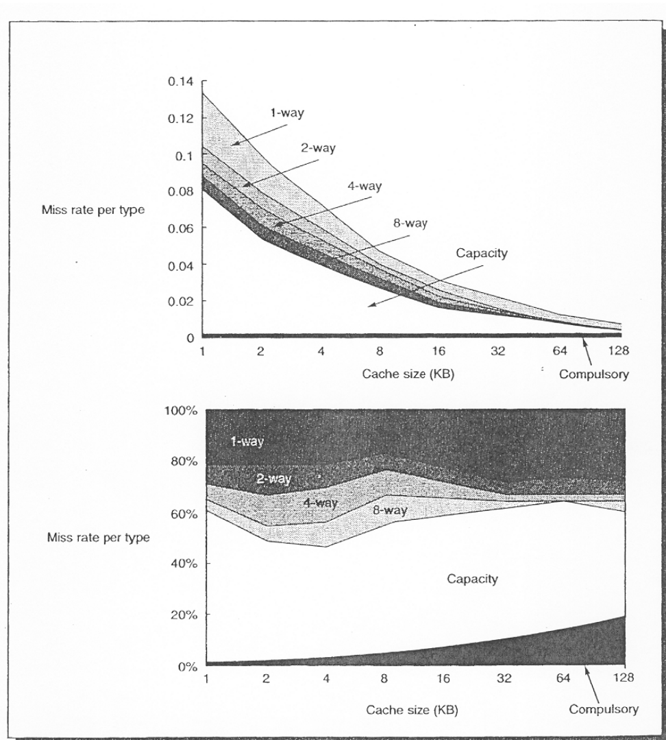
Total miss rate (top) and distribution of miss rate (bottom) for each size cache according to three C's for the data in Figure 5.9. The top diagram is the actual miss rates, while the bottom diagram is scaled to the direct-mapped miss ratios.
